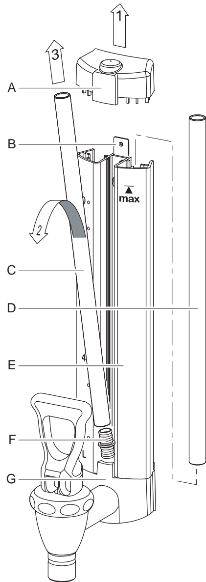
Cleaning gauge glass
