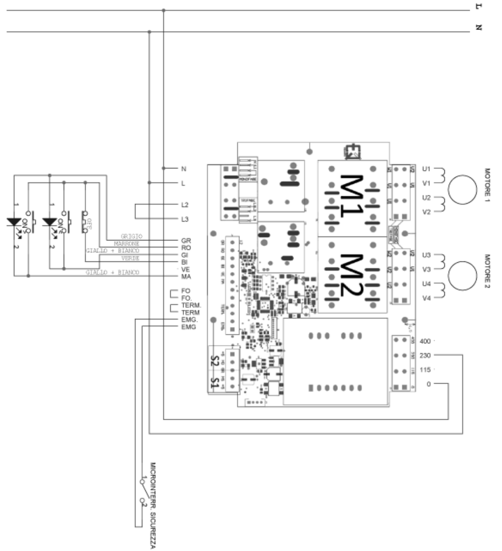
- Single-phase wiring diagram of stainless steel controls
